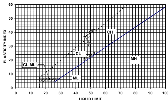
Unified Soil Classification System Plasticity Chart
