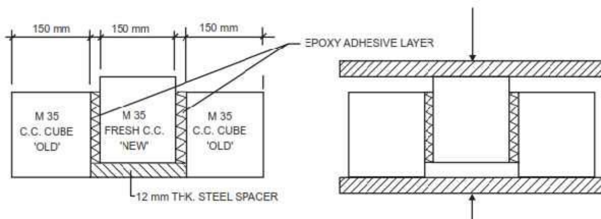
Fig 27.1: Bonding test arrangement of Epoxy
