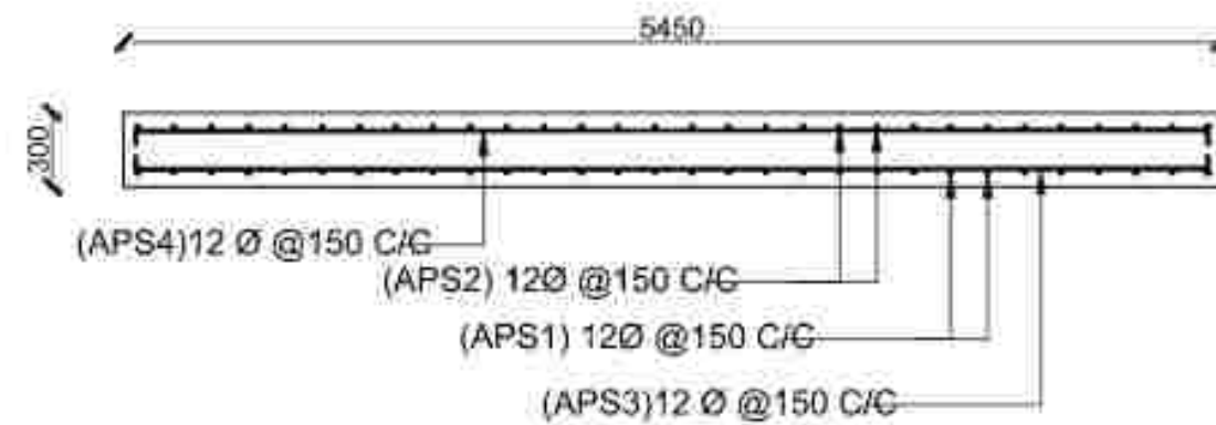
Approach Slab Rebar Section
