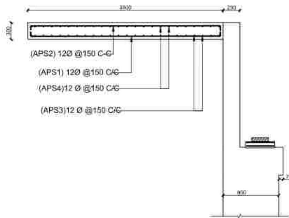
Approach Slab Rebar Section and Its Arrangement on Dirt Wall
