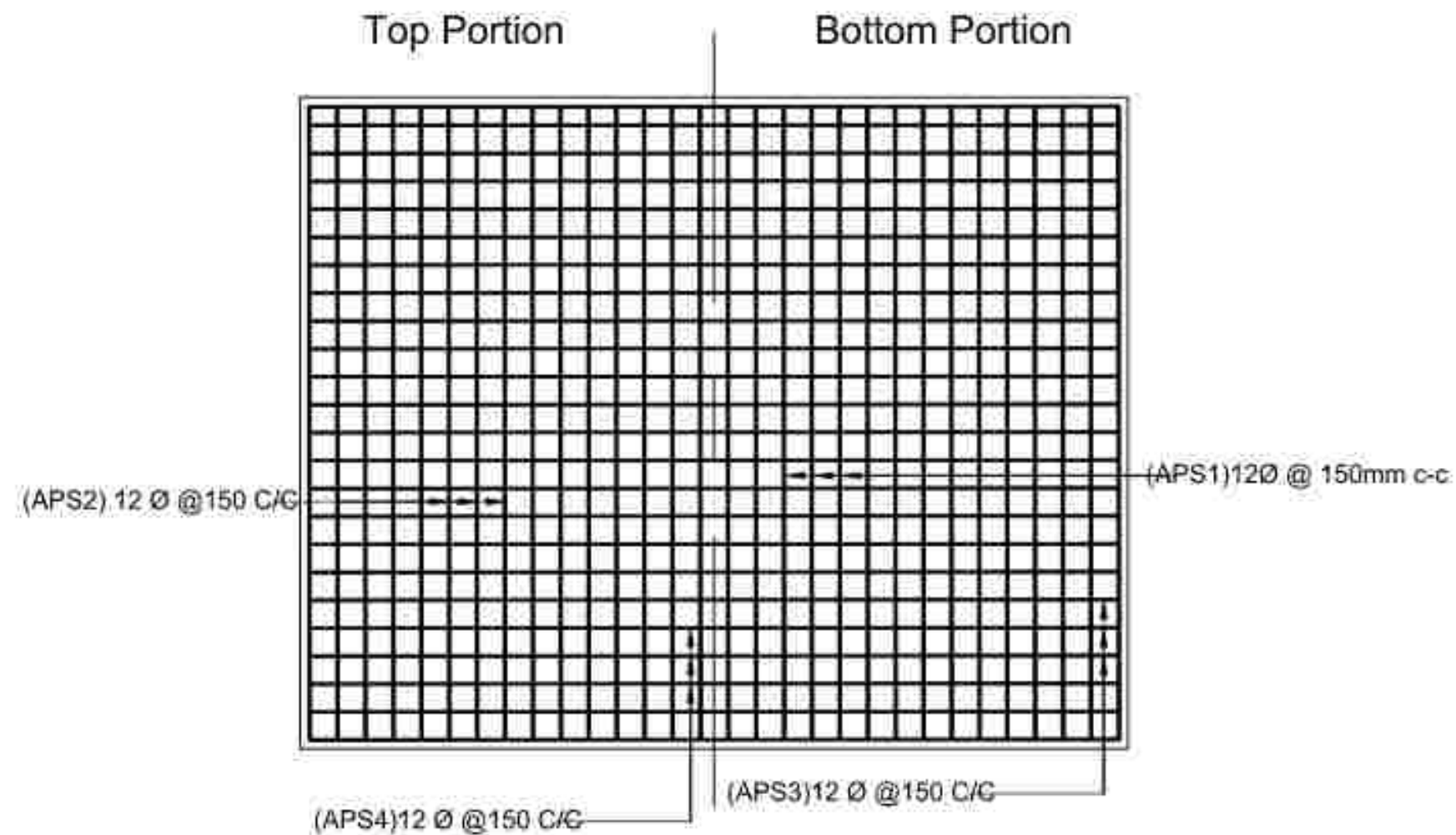
Approach Slab Rebar Arrangement Plan
