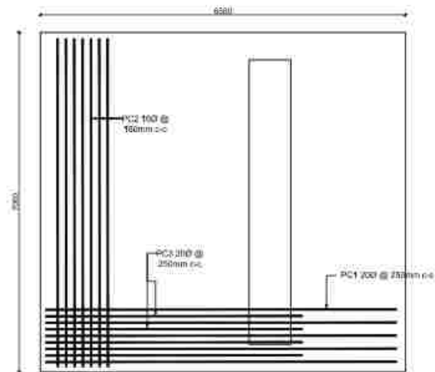
Footing Bottom Reinforcement Details
