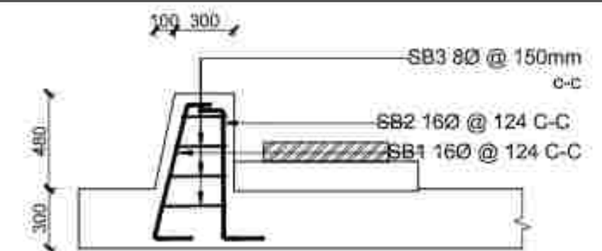
Stopper Block Rebar Arrangement Section
