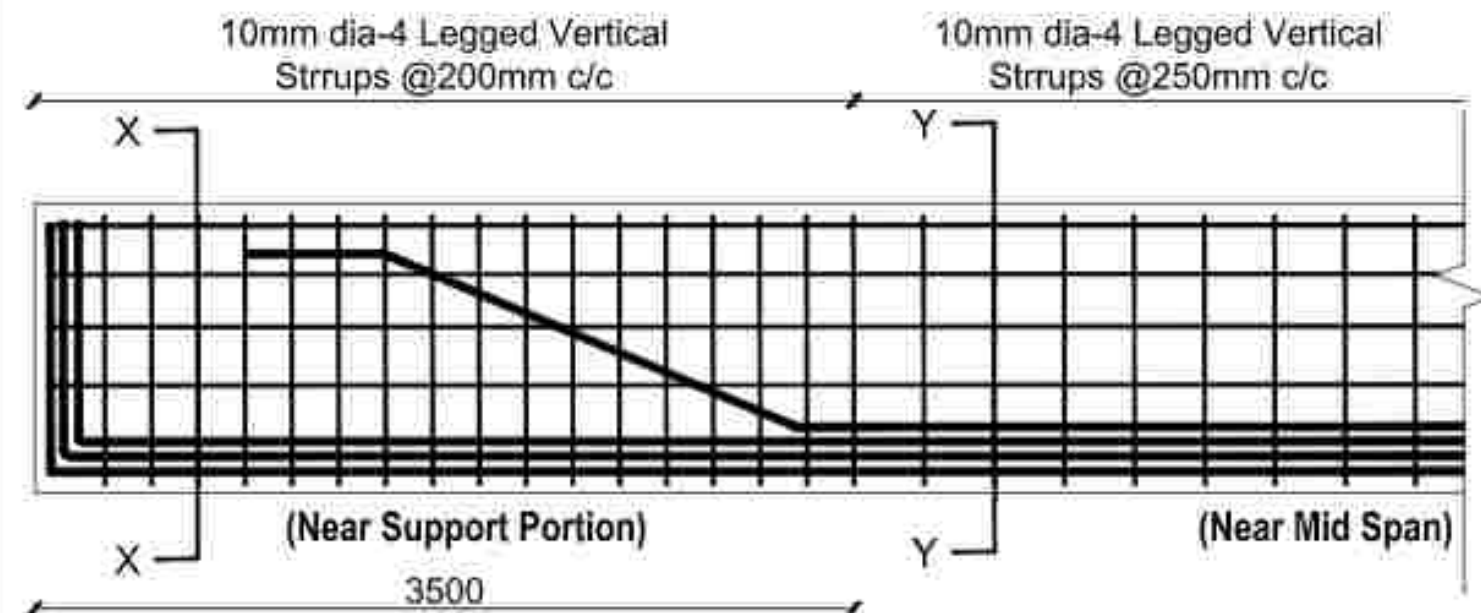
LONGITUDINAL SECTION OF MAIN BEAM
