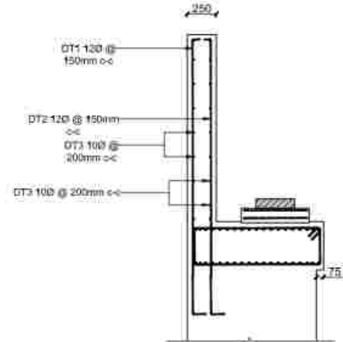
Abutment Cap and Dirt Wall Rebar Arrangement Section
