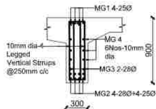
SECTION Y-Y (Cross Section of Main Girder near Mid Span)
