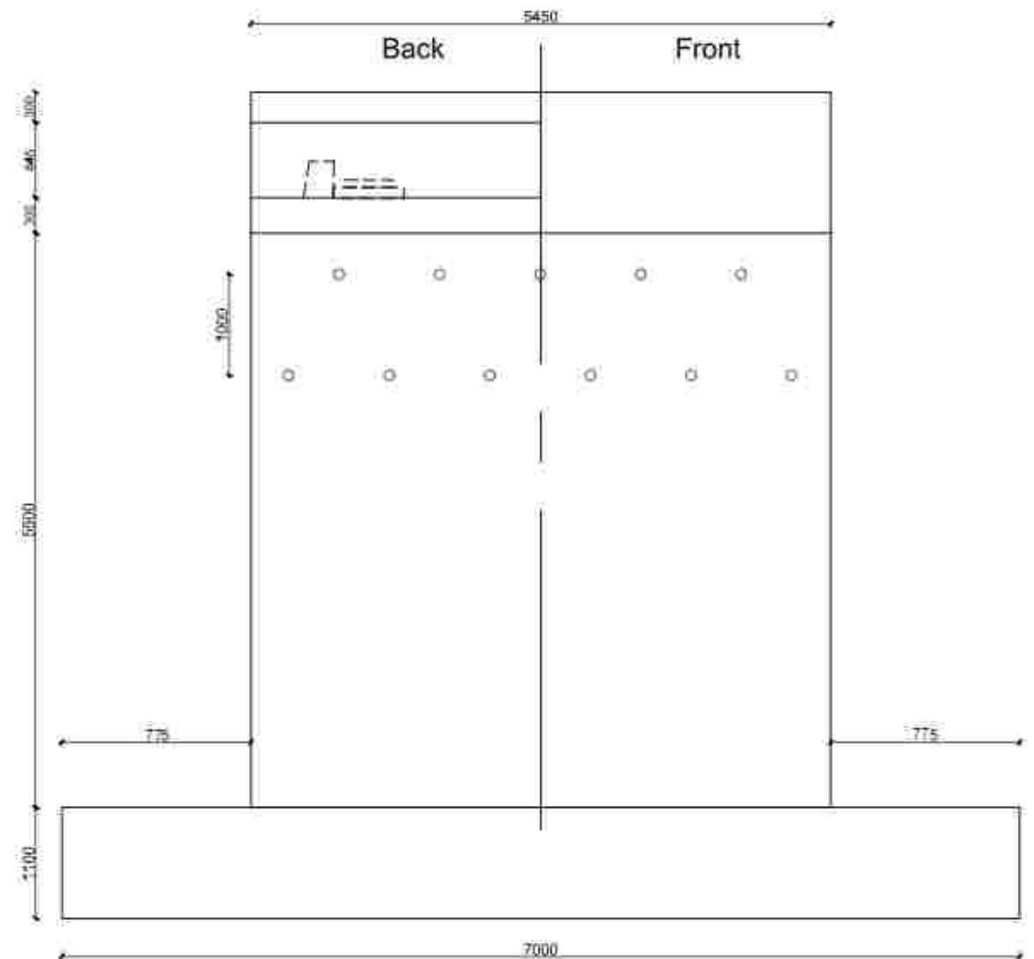
Abutment Longitudinal Section
