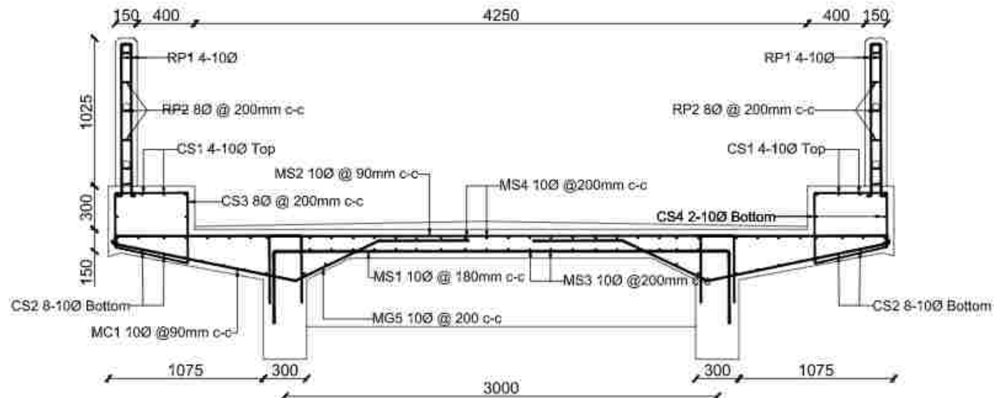
DECK SLAB CROSS SECTION WITH REBAR ARRANGEMENT (With Reinforcement Details)
