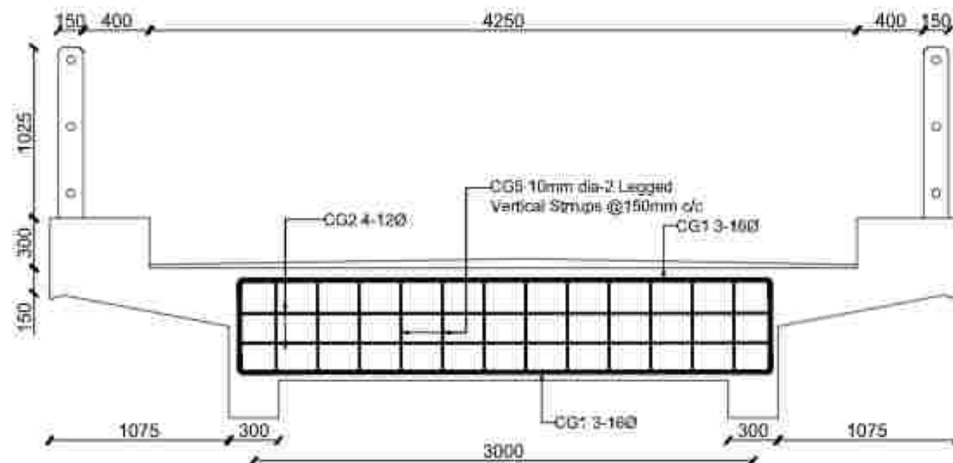
LONGITUDINAL SECTION OF END/ INTERMEDIATE CROSS GIRDER (With Reinforcement Details)
