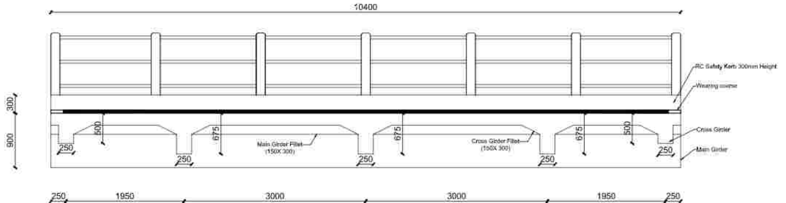
BRIDGE LONGITUDINAL SECTION
