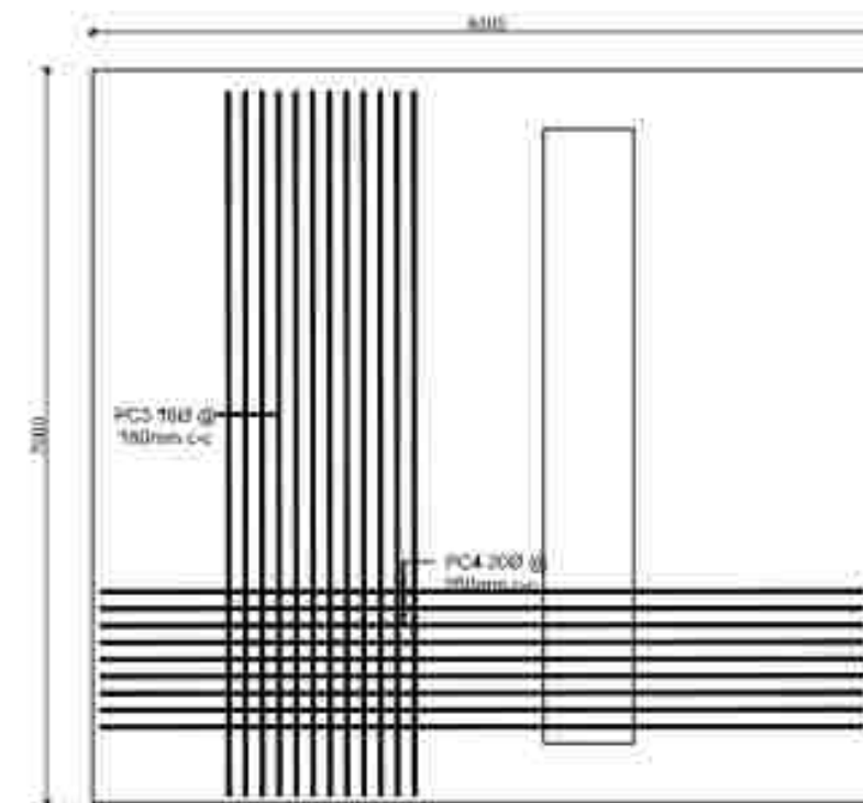
Footing Top Reinforcement Details
