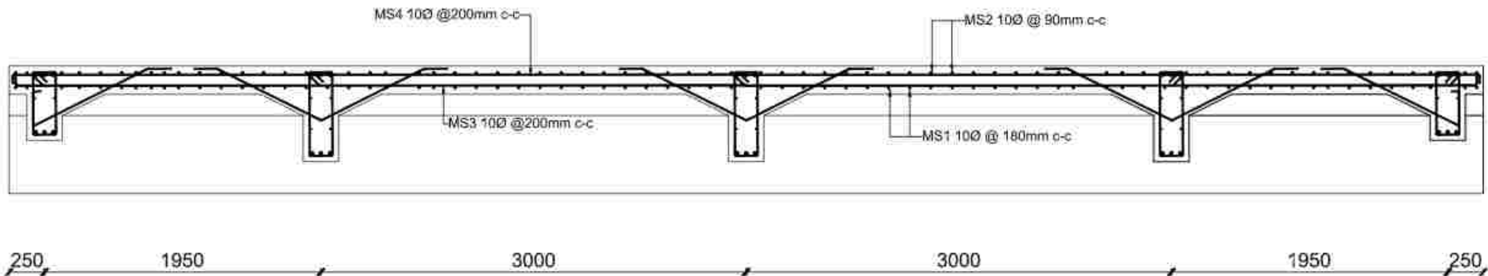
BRIDGE LONGITUDINAL SECTION (With Reinforcement Details)
