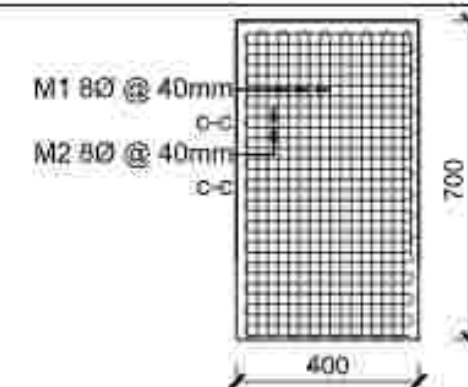
Bearing Pedestal Reinforcement Plan
