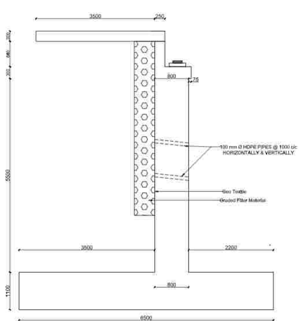
Abutment Cross Section
