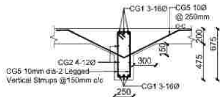
CROSS SECTION OF INTERMEDIATE CROSS GIRDER
