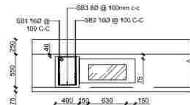
Stopper Block Rebar Arrangement Plan
