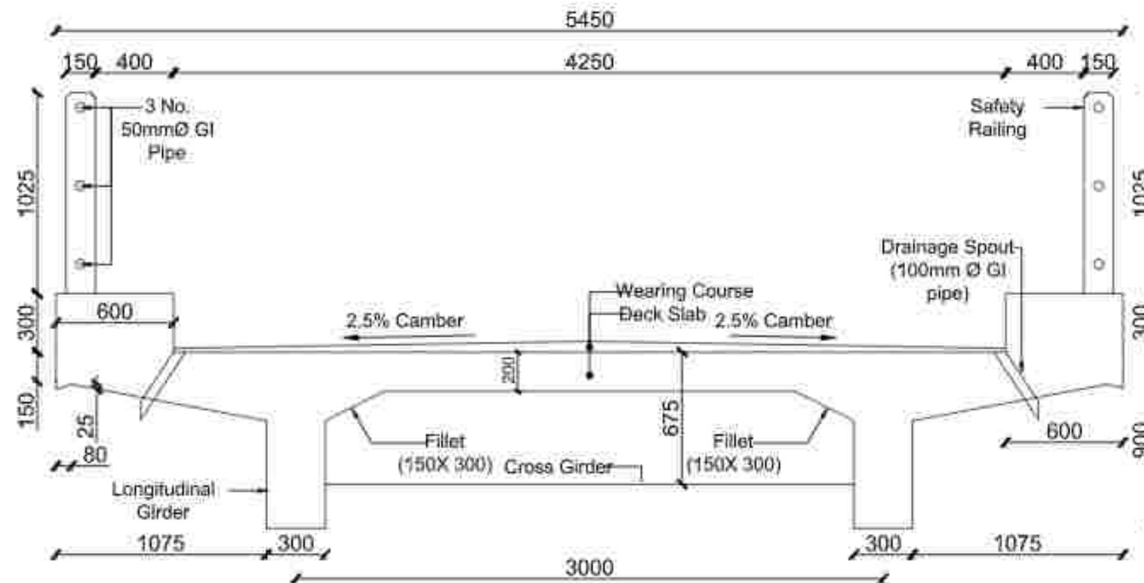
DECK CROSS SECTION
