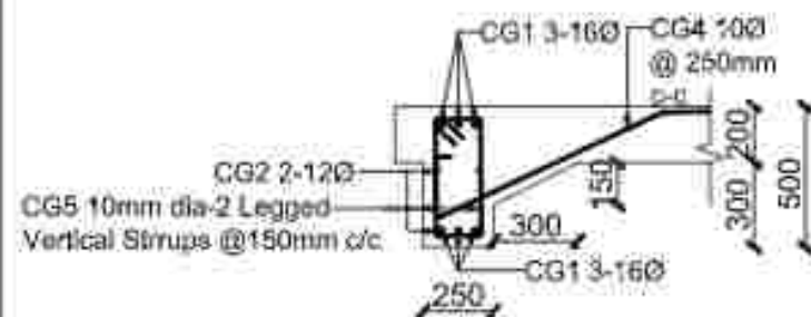
SECTION X-X (Cross Section of Main Girder near Support)
