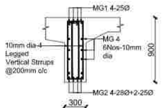
SECTION X-X (Cross Section of Main Girder near Support)
